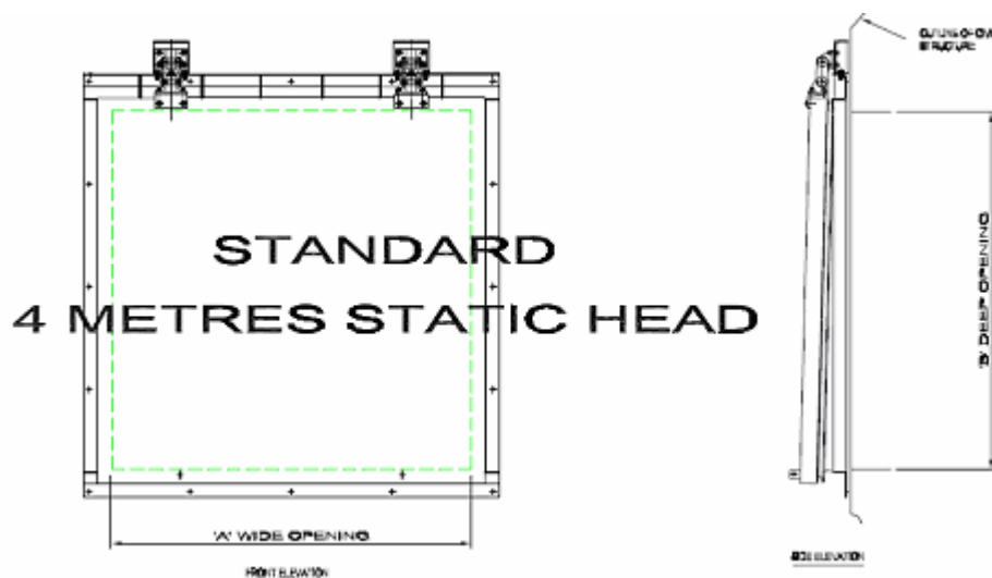
Figure 7.22: Double-hung flap valve (plastic door)
